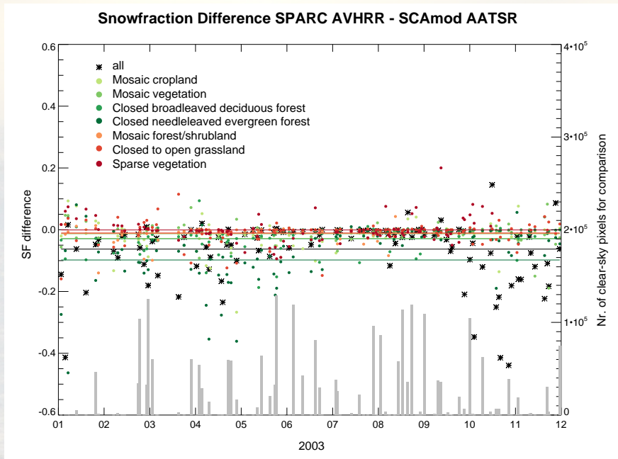
Figure 10: SCA differences between the two snow detection schemes (AATSR SCAMod and AVHRR SPARC for 2003 over the European Alps. Data points are displayed for days when a minimum of 500 coincident clear-sky pixels were available. Overall difference is given in black while the smaller colored dots refer to specific landcover classes (see legend). Lines indicate overall mean of the given landcover class and grey bars show the amount of pixels available for comparison.
