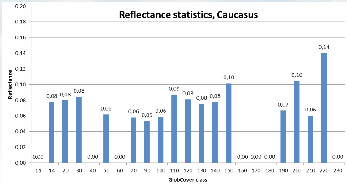
Figure 6: Mean reflectance values calculated for the GlobCover classes.
