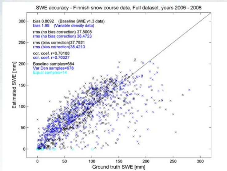
Figure 4: SWE retrieval comparison between the baseline GlobSnow-1 v1.3 SWE and the variable density datasets acquired using Finnish snow course data.
