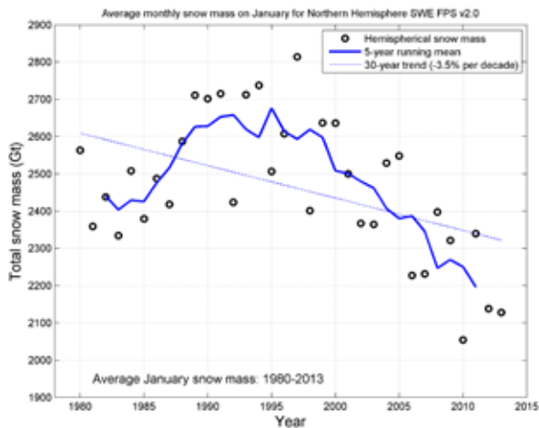
Figure 2: The long term trends, based on GlobSnow SWE v2.0 monthly data, for Northern Hemisphere for 1980 - 2013.”
