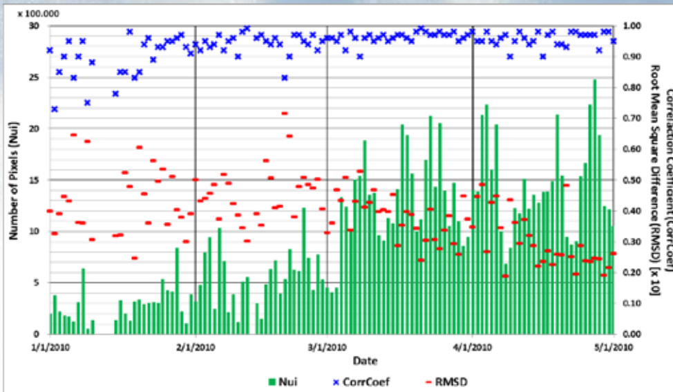
Figure 6: Statistical parameters Number of pixels (green bars), Root Mean Square Difference (RMSD) (red dots) and Correlation Coefficient (blue crosses) resulting from the daily intercomparison of the GlobSnow-2 version 2.0 SE product with the fractional snow cover product of the EU FP7 project CryoLand covering the area 72N/11W to 35N/50E with about 500 m grid size for the period 1st of January 2010 to 1st of May 2010.
