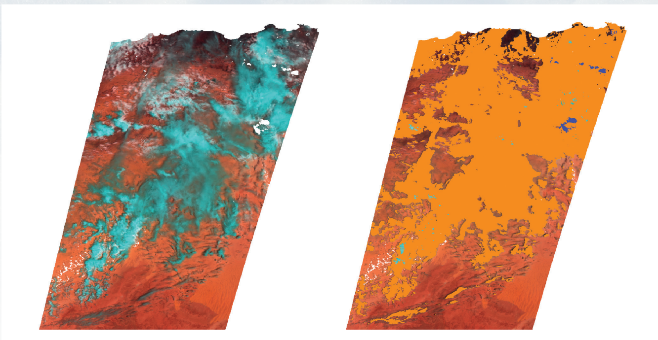
Figure 4: Evaluation of cloud masks retrieved by the SCDA algorithm. The left image shows an RGB colour composite based on AATSR bands at 1600, 670 and 550 nm for Algeria on 25 May 2003. The image on the right shows the SCDA cloud mask in orange put on top of the image at the left. The agreement is very good in general. However, a few cold cloud tops could not be detected (dots in cyan in the right image).
