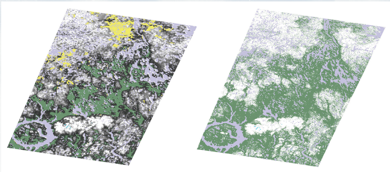
Figure 5: Comparison between GlobSnow fractional snow cover map (left) and a binary snow map derived from a Landsat 7 ETM+ scene for comparison (right). The area is in the north-east Canada, and images were acquired on 15 May 2003.
