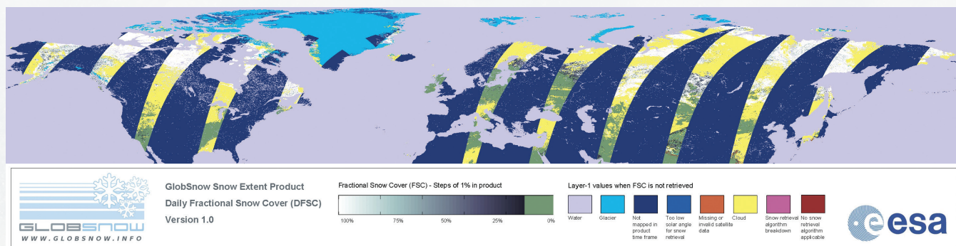
Figure 6: GlobSnow Fractional Snow Cover (FSC) product sample ('quick-look' image) based on all Envisat AATSR acquisitions in the Northern Hemisphere on 1 April 2007.
