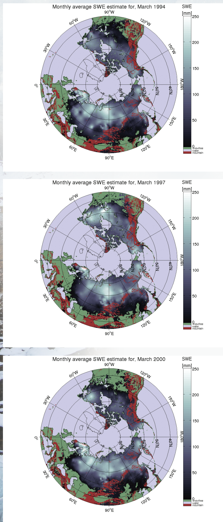
Figure 3: Monthly average of SWE estimate in the Northern Hemisphere for March 1994, 1997 and 2000.
