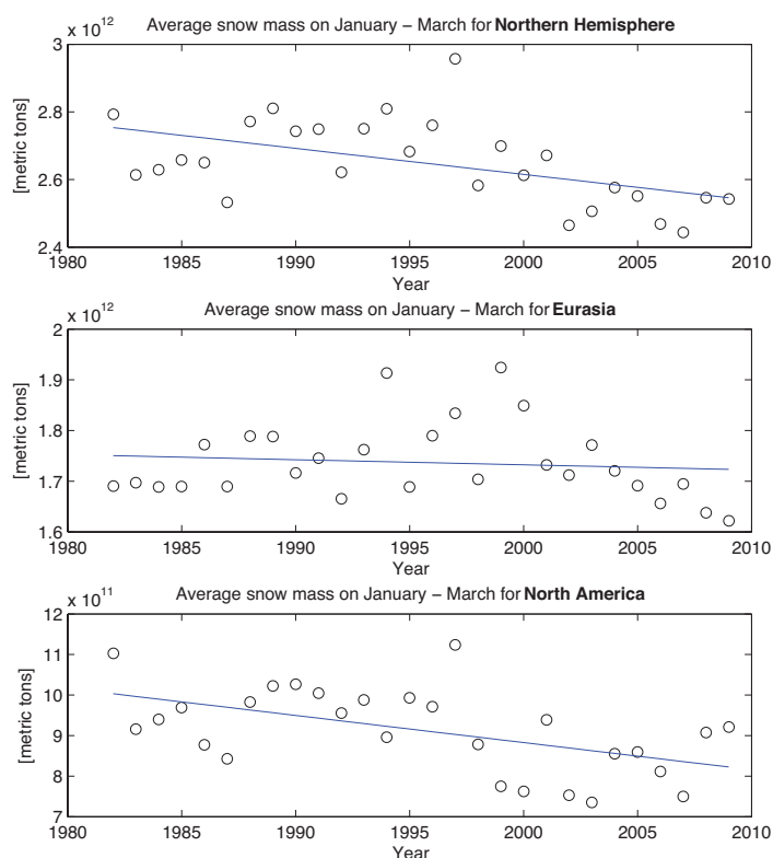
Figure 2: Average snow mass and trends for the winter period January-March 1982-2009 for the Northern Hemisphere, Eurasia and North America.
