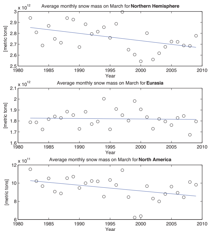
Figure 1: Average monthly snow mass and trends for March 1982-2009 for the Northern Hemisphere, Eurasia and North America.
