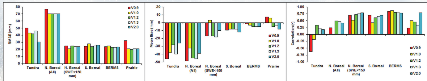
Figure 3: The evaluation of various GlobSnow SWE datasets with Canadian reference data. The left panel shows the Root-Mean-Squared-Error for different datasets, center panel shows the mean bias and right panel shows the correlation coefficients between SWE datasets and the reference data.
